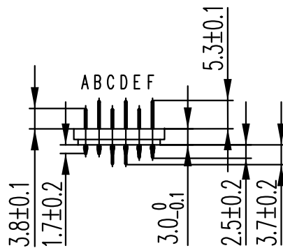
Contact selection options, male contacts
