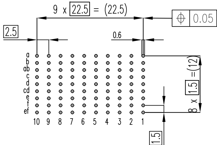
PCB LAYOUT
