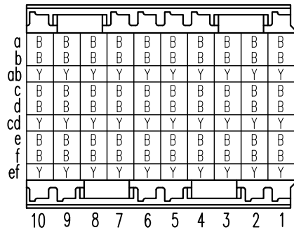
CONTACT LAYOUT
