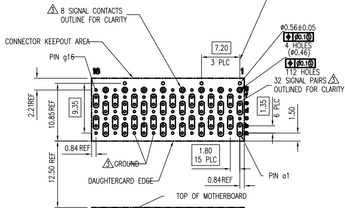
PC BOARD LAYOUT (CONNECTOR SIDE)
